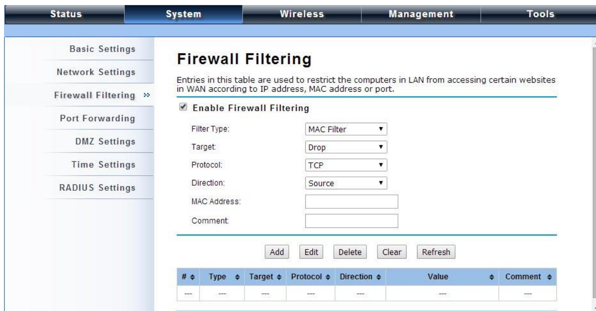
Figure 13 Source IP Filtering
