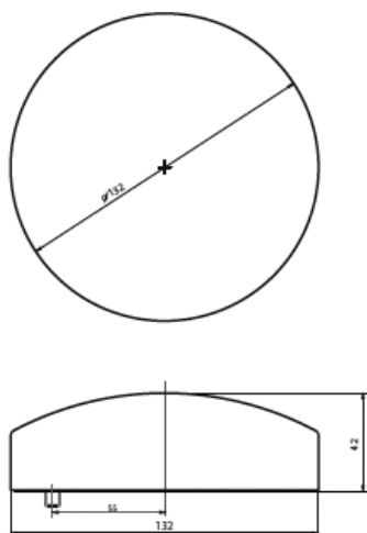
Dimensions (mm)
