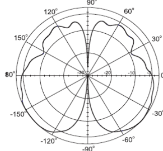
Vertical Pattern @ 2.4 GHz
